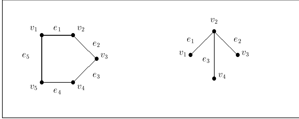
Figure 2.1: A loop and a tree.
